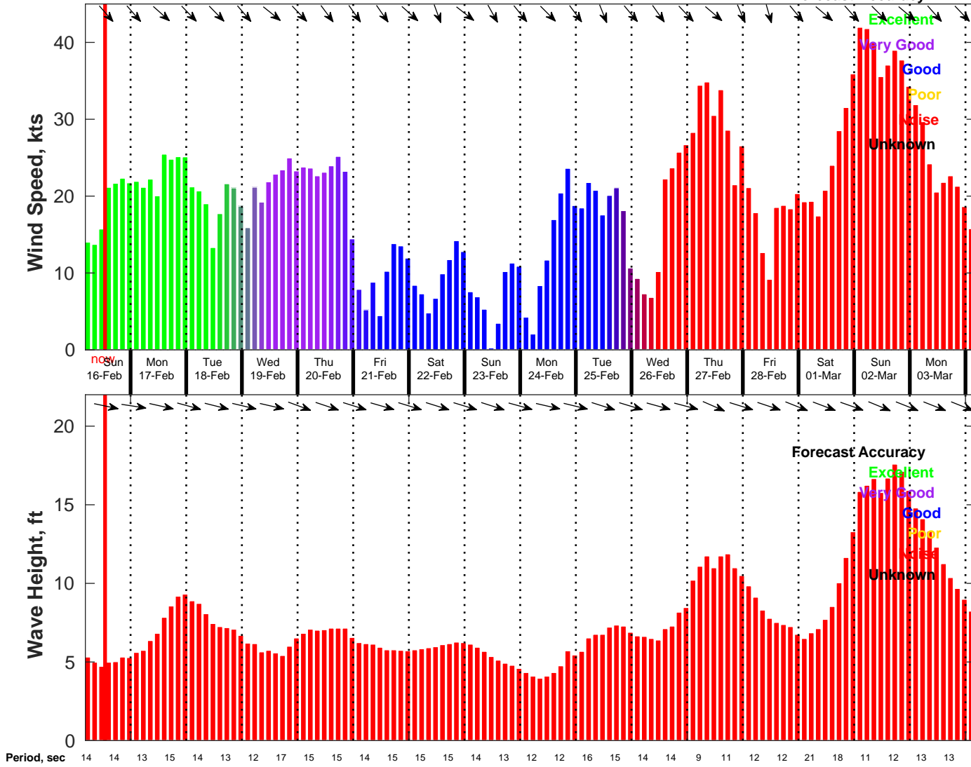
Wind & Wave Forecast for NDBC 46054 from 16-Feb-2025 04:00:00 to 04-Mar-2025 04:00:00
