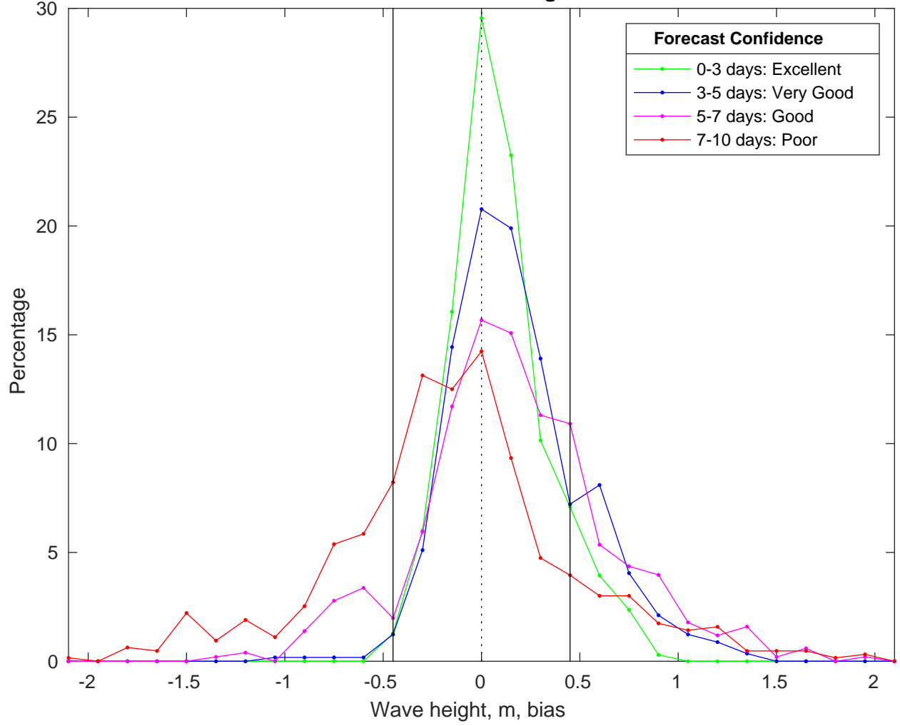
NDBC 46069 vs CMEMS Waves Bias Histogram: 16-Feb-2025
