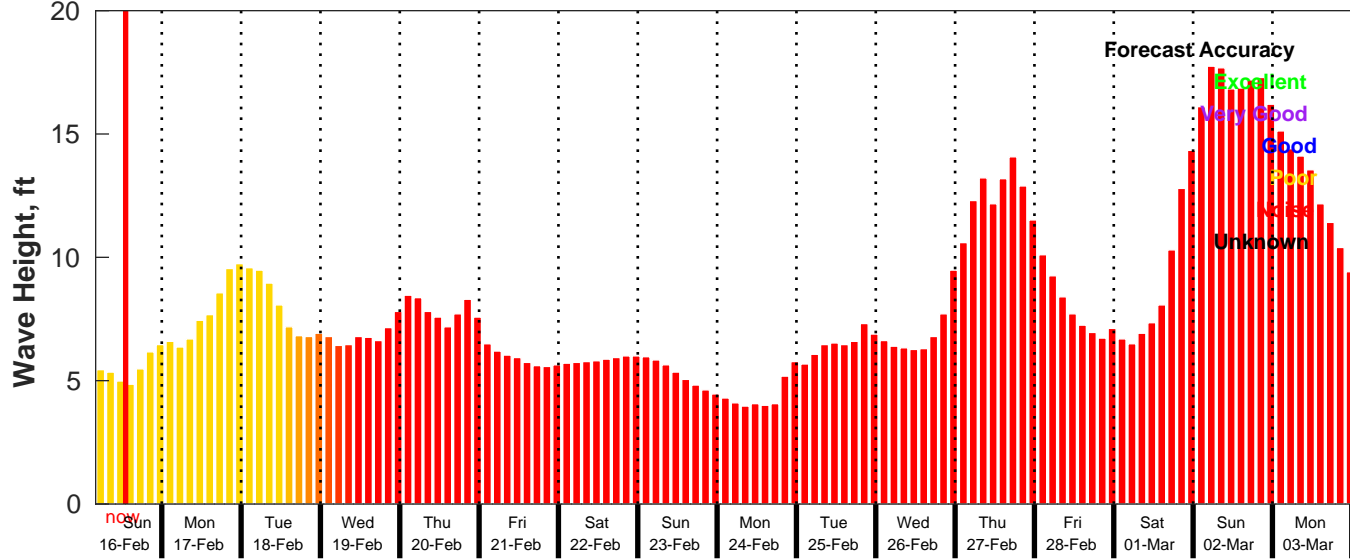
GFS Wave Forecast for NDBC 46069 from 16-Feb-2025 04:00:00 to 04-Mar-2025 04:00:00
