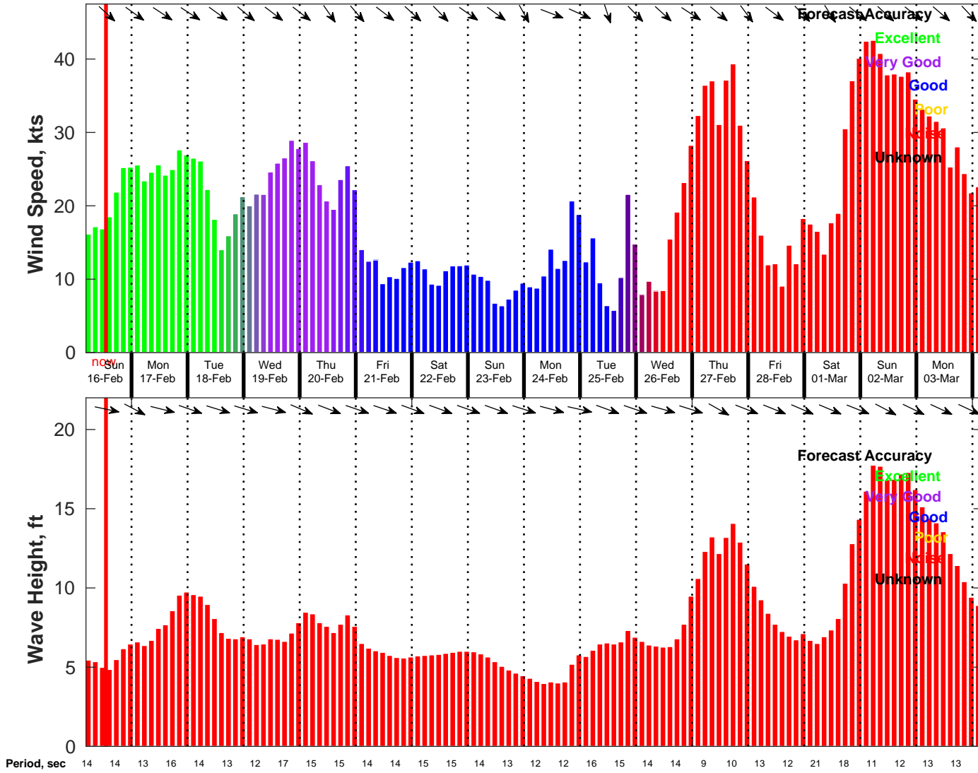
Wind & Wave Forecast for NDBC 46069 from 16-Feb-2025 04:00:00 to 04-Mar-2025 04:00:00
