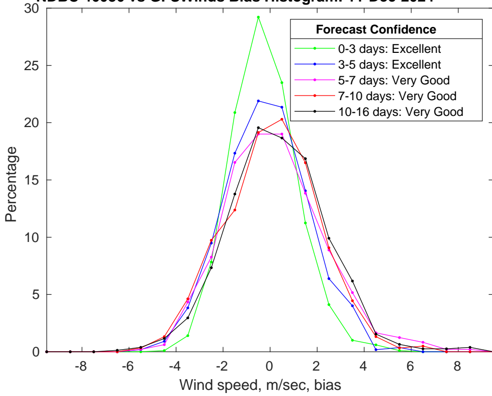
NDBC 46086 vs GFSWinds Bias Histogram: 11-Dec-2024
