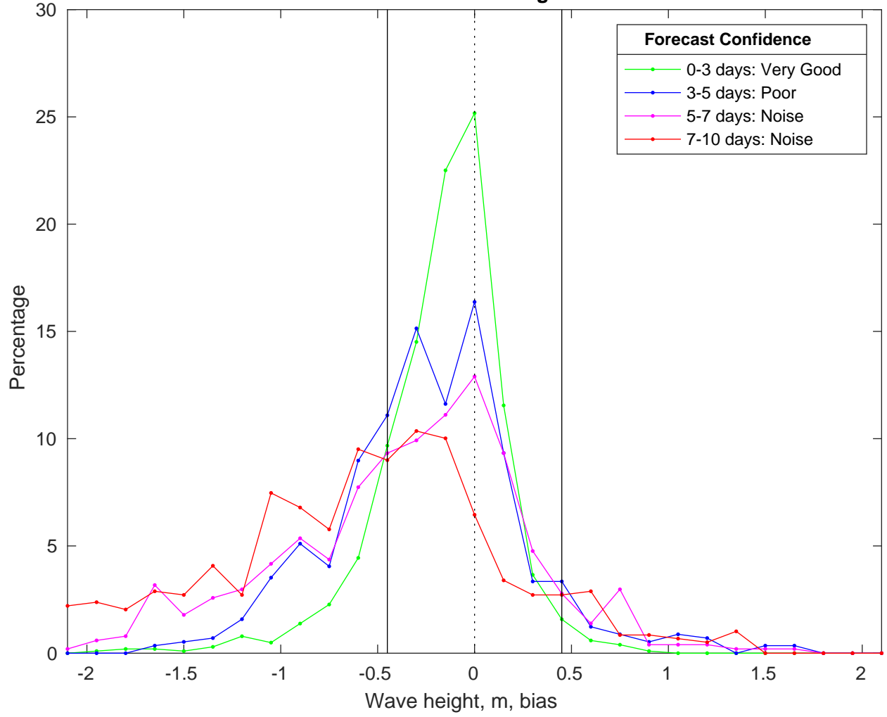
NDBC 46246 vs CMEMS Waves Bias Histogram: 16-Feb-2025
