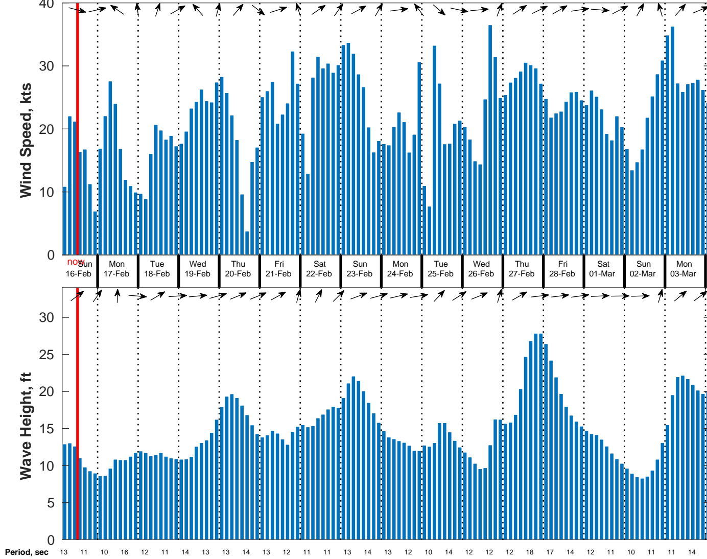
Wind & Wave Forecast for NDBC 46246 from 16-Feb-2025 03:00:00 to 04-Mar-2025 03:00:00
