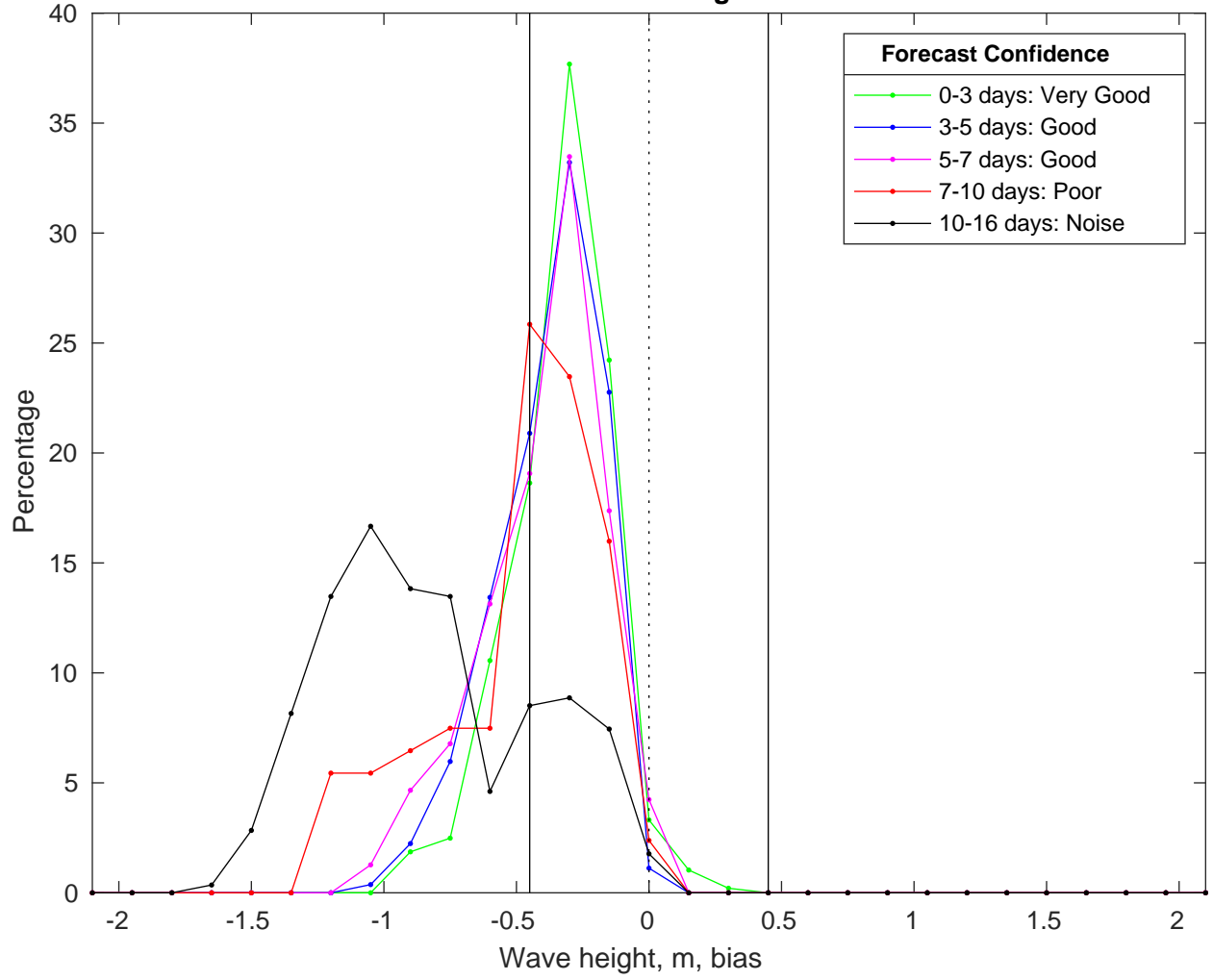
NDBC 51209 vs GFS Waves Bias Histogram: 16-Feb-2025
