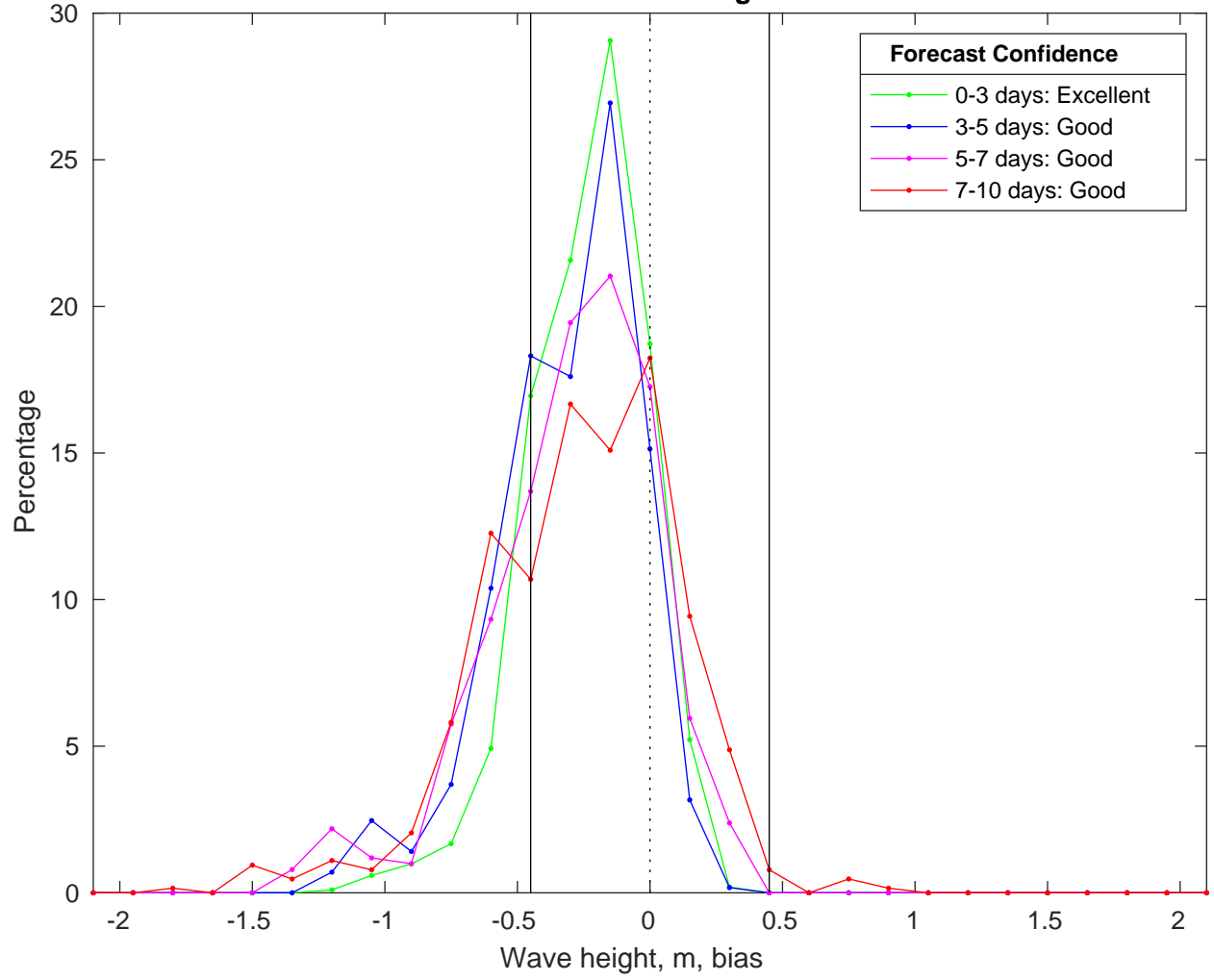
NDBC 52211 vs CMEMS Waves Bias Histogram: 16-Feb-2025
