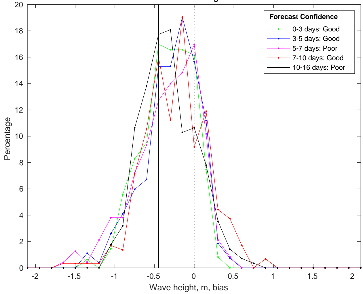
NDBC 52211 vs GFS Waves Bias Histogram: 16-Feb-2025
