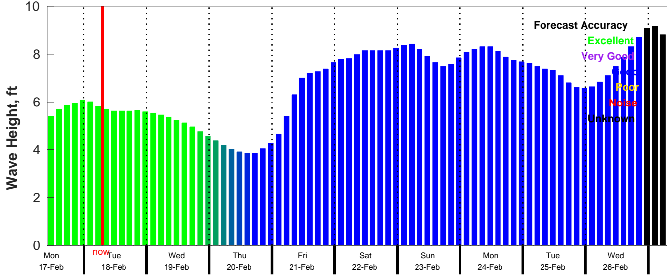
CMEMS Wave Forecast for NDBC 52211 from 16-Feb-2025 10:00:00 to 26-Feb-2025 10:00:00
