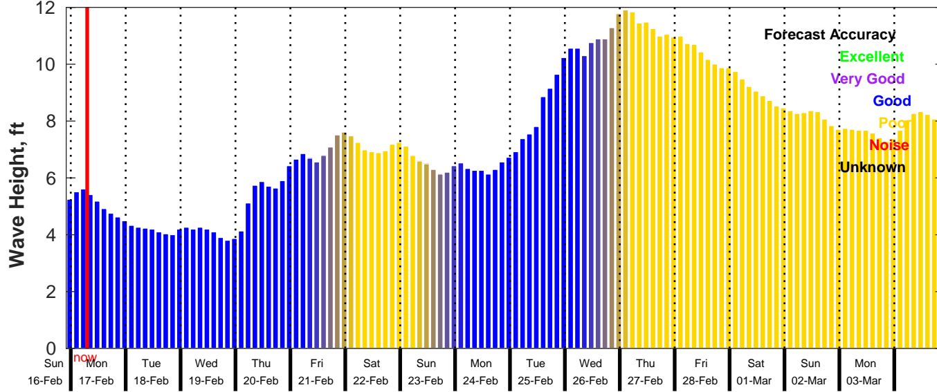
GFS Wave Forecast for NDBC 52211 from 16-Feb-2025 22:00:00 to 04-Mar-2025 22:00:00
