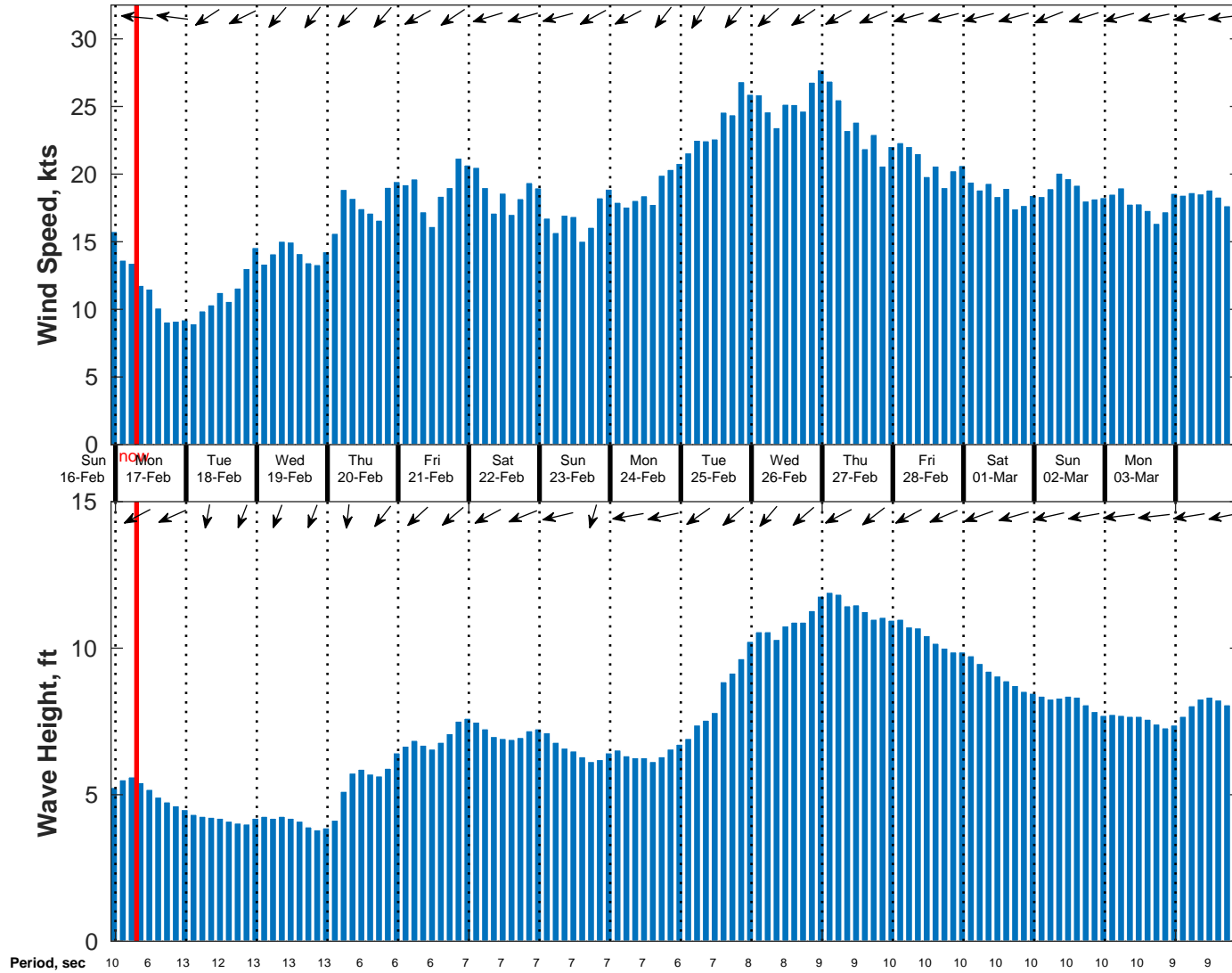
Wind & Wave Forecast for NDBC 52211 from 16-Feb-2025 22:00:00 to 04-Mar-2025 22:00:00
