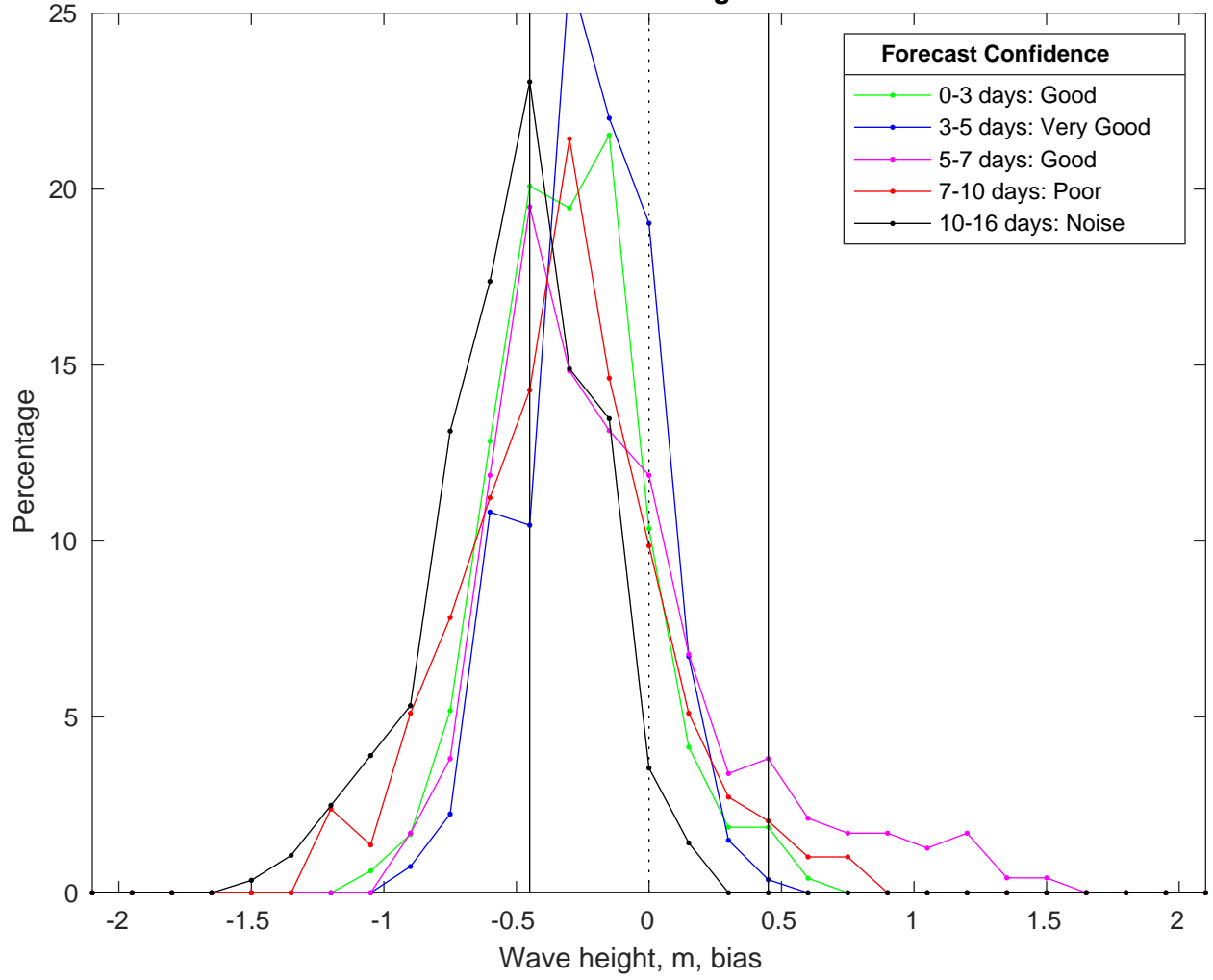
NDBC 52212 vs GFS Waves Bias Histogram: 16-Feb-2025
