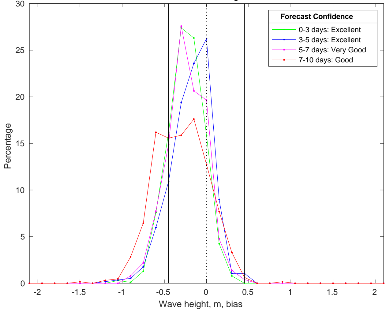
NDBC 52213 vs CMEMS Waves Bias Histogram: 16-Feb-2025
