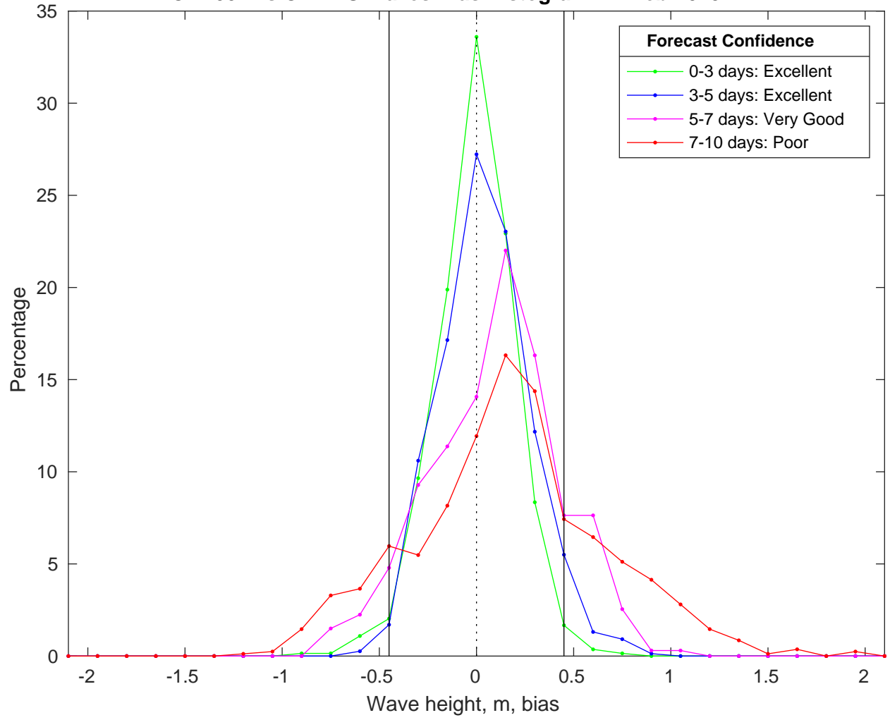
NDBC 41004 vs CMEMS Waves Bias Histogram: 17-Feb-2025
