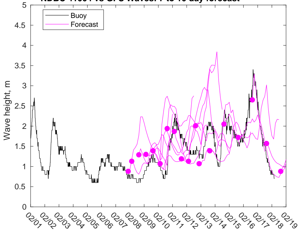
NDBC 41004 vs GFS Waves: 7 to 10 day forecast
