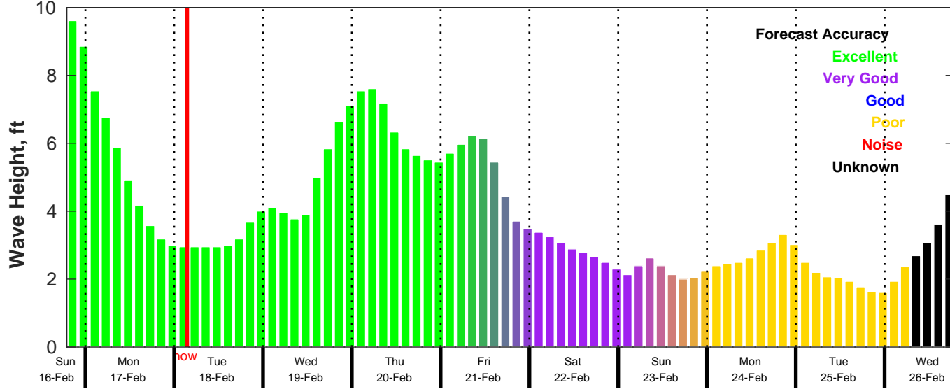
CMEMS Wave Forecast for NDBC 41004 from 16-Feb-2025 19:00:00 to 26-Feb-2025 19:00:00
