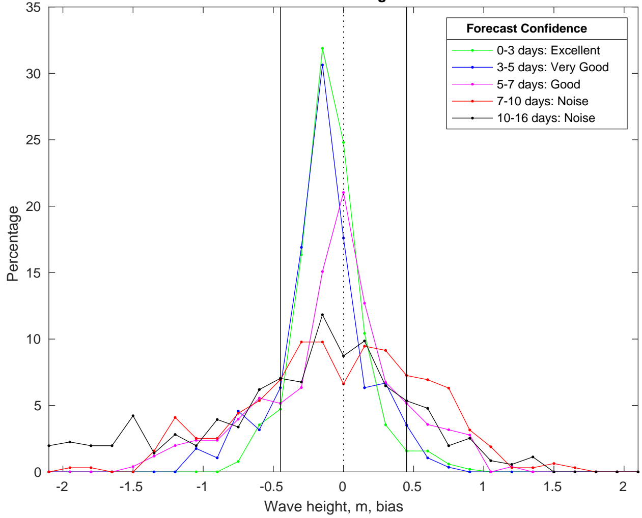
NDBC 41013 vs GFS Waves Bias Histogram: 17-Feb-2025
