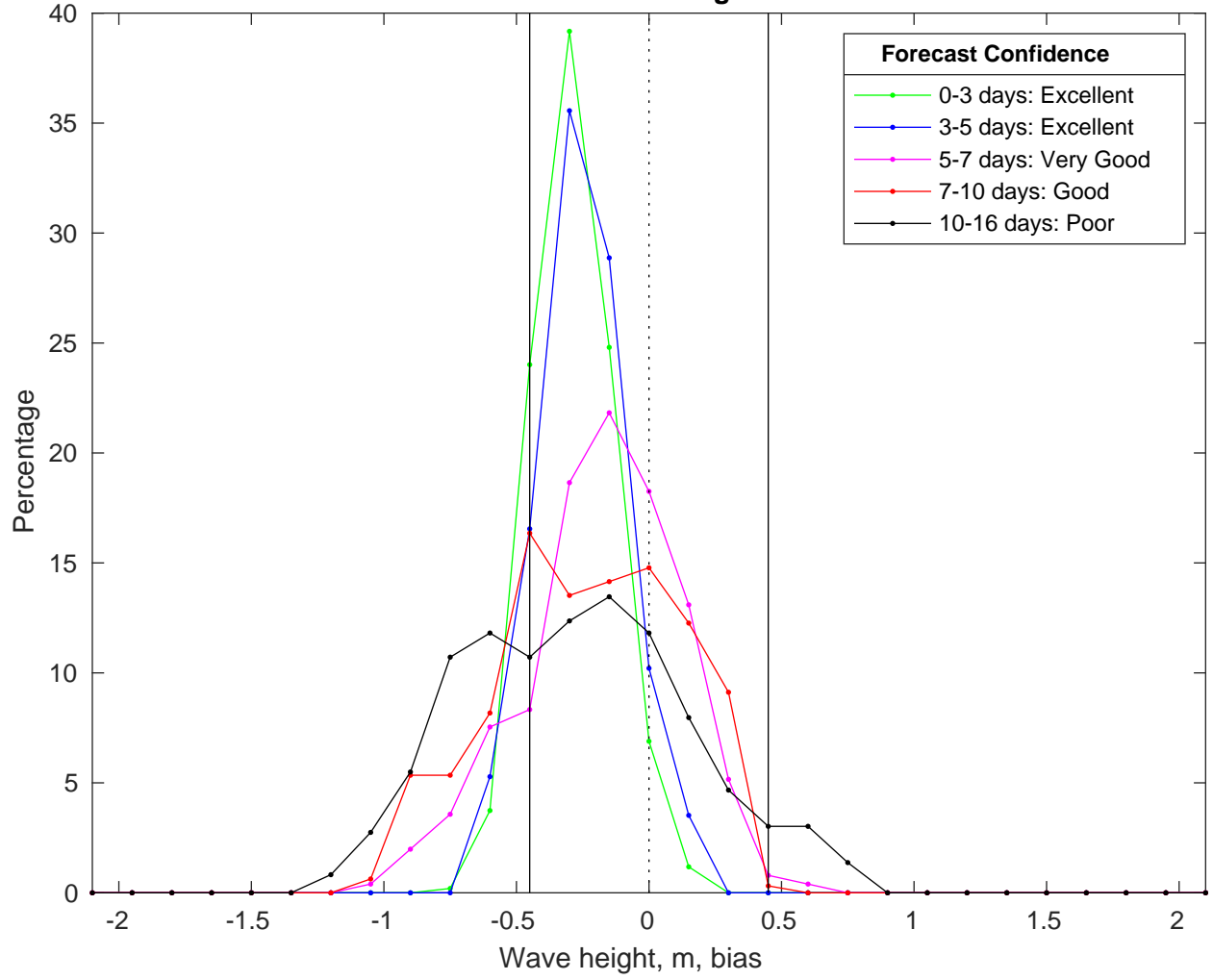
NDBC 41040 vs GFS Waves Bias Histogram: 17-Feb-2025
