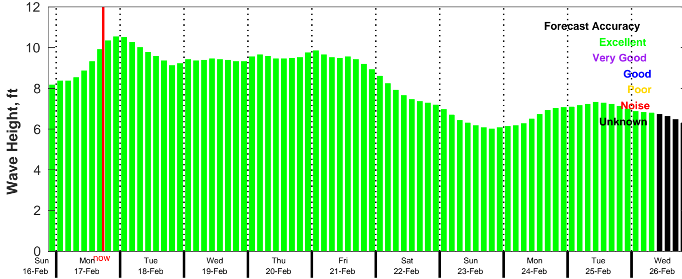
CMEMS Wave Forecast for NDBC 41040 from 16-Feb-2025 21:00:00 to 26-Feb-2025 21:00:00
