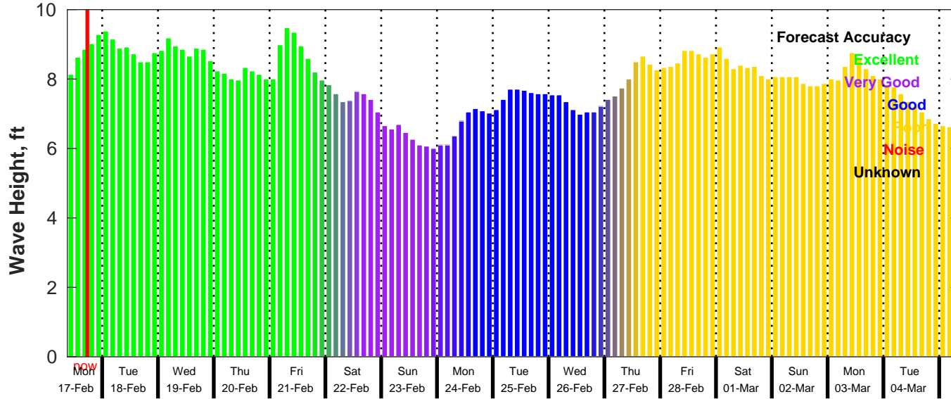
GFS Wave Forecast for NDBC 41040 from 17-Feb-2025 09:00:00 to 05-Mar-2025 09:00:00
