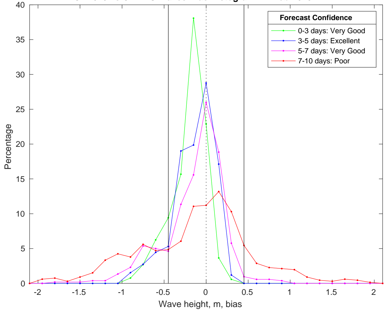
NDBC 42019 vs CMEMS Waves Bias Histogram: 17-Feb-2025
