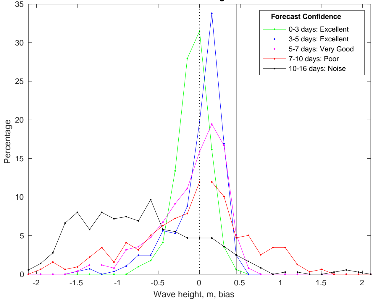
NDBC 42019 vs GFS Waves Bias Histogram: 17-Feb-2025
