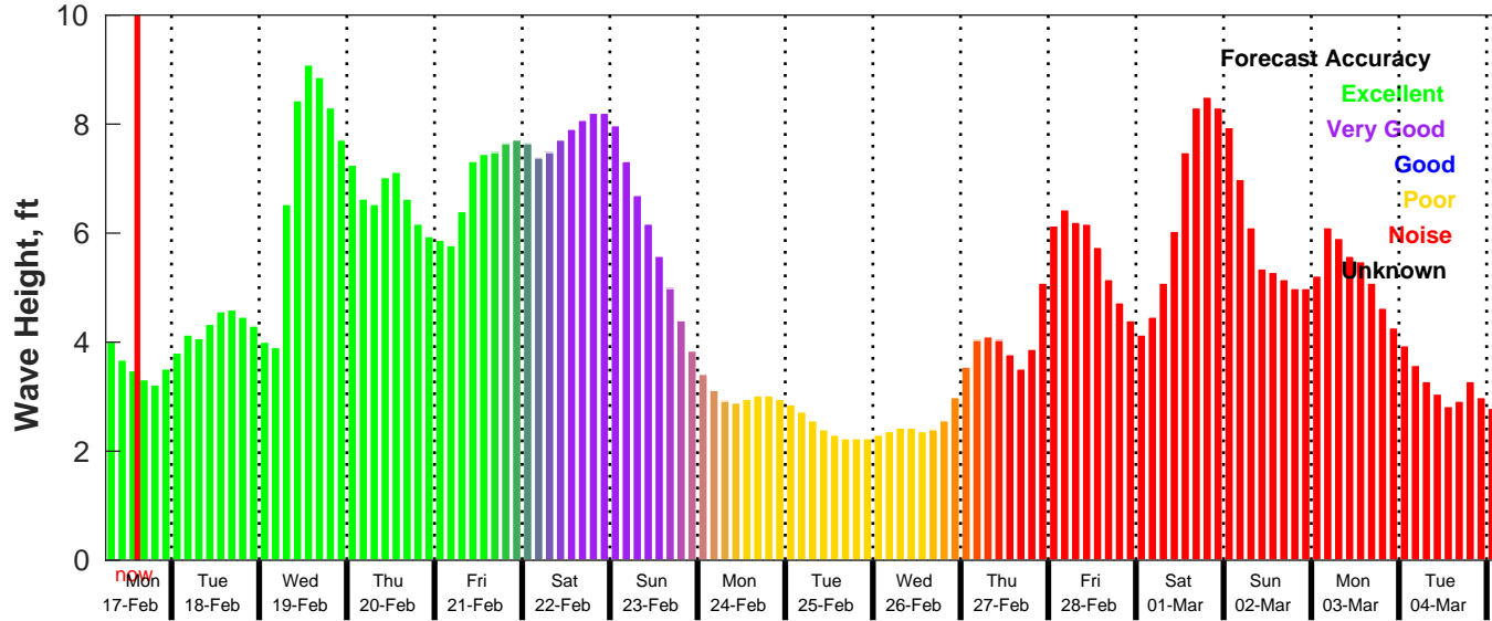
GFS Wave Forecast for NDBC 42019 from 17-Feb-2025 06:00:00 to 05-Mar-2025 06:00:00
