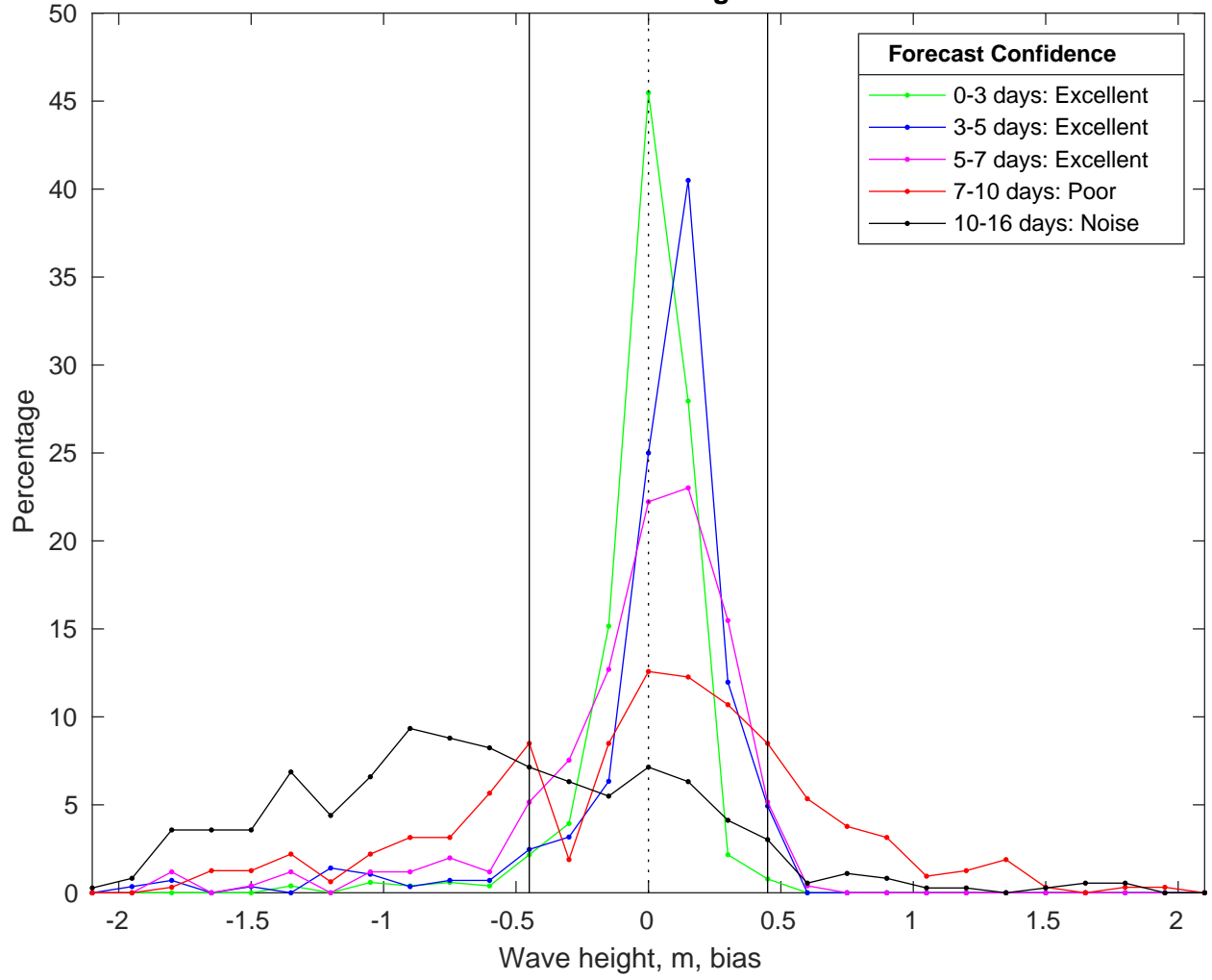
NDBC 42020 vs GFS Waves Bias Histogram: 17-Feb-2025
