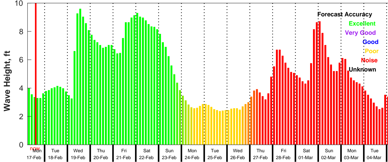
GFS Wave Forecast for NDBC 42020 from 17-Feb-2025 06:00:00 to 05-Mar-2025 06:00:00
