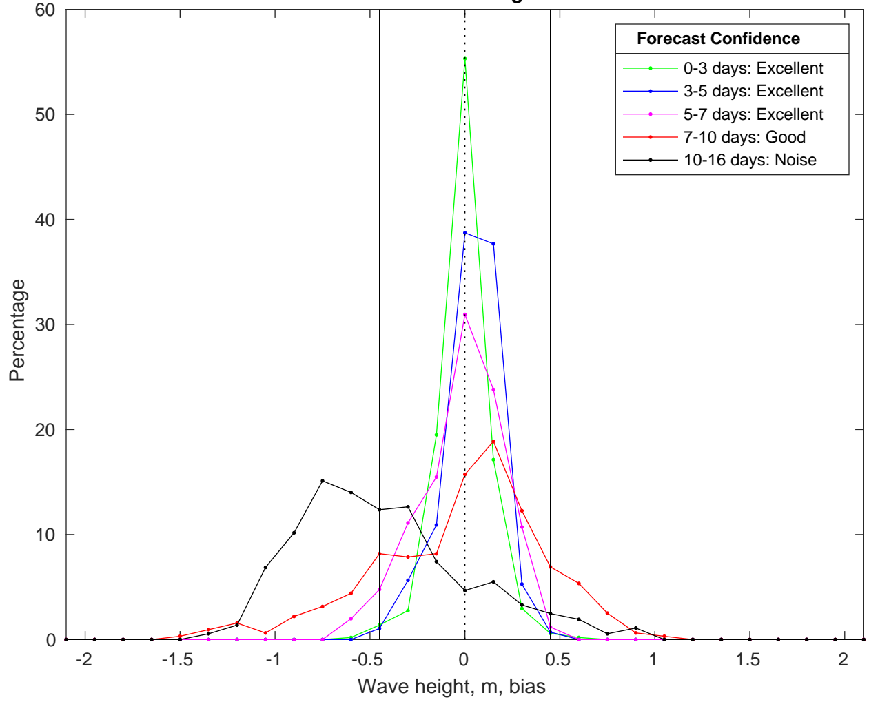
NDBC 42035 vs GFS Waves Bias Histogram: 17-Feb-2025
