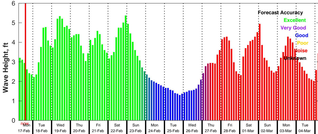
GFS Wave Forecast for NDBC 42035 from 17-Feb-2025 06:00:00 to 05-Mar-2025 06:00:00
