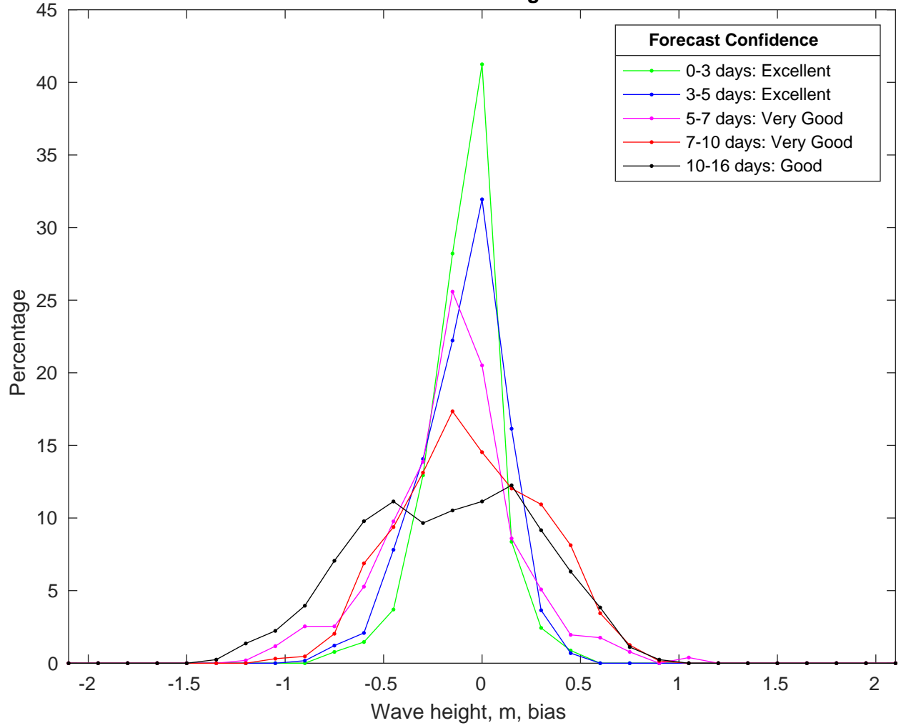
NDBC 42035 vs GFSWaves Bias Histogram: 26-Dec-2024
