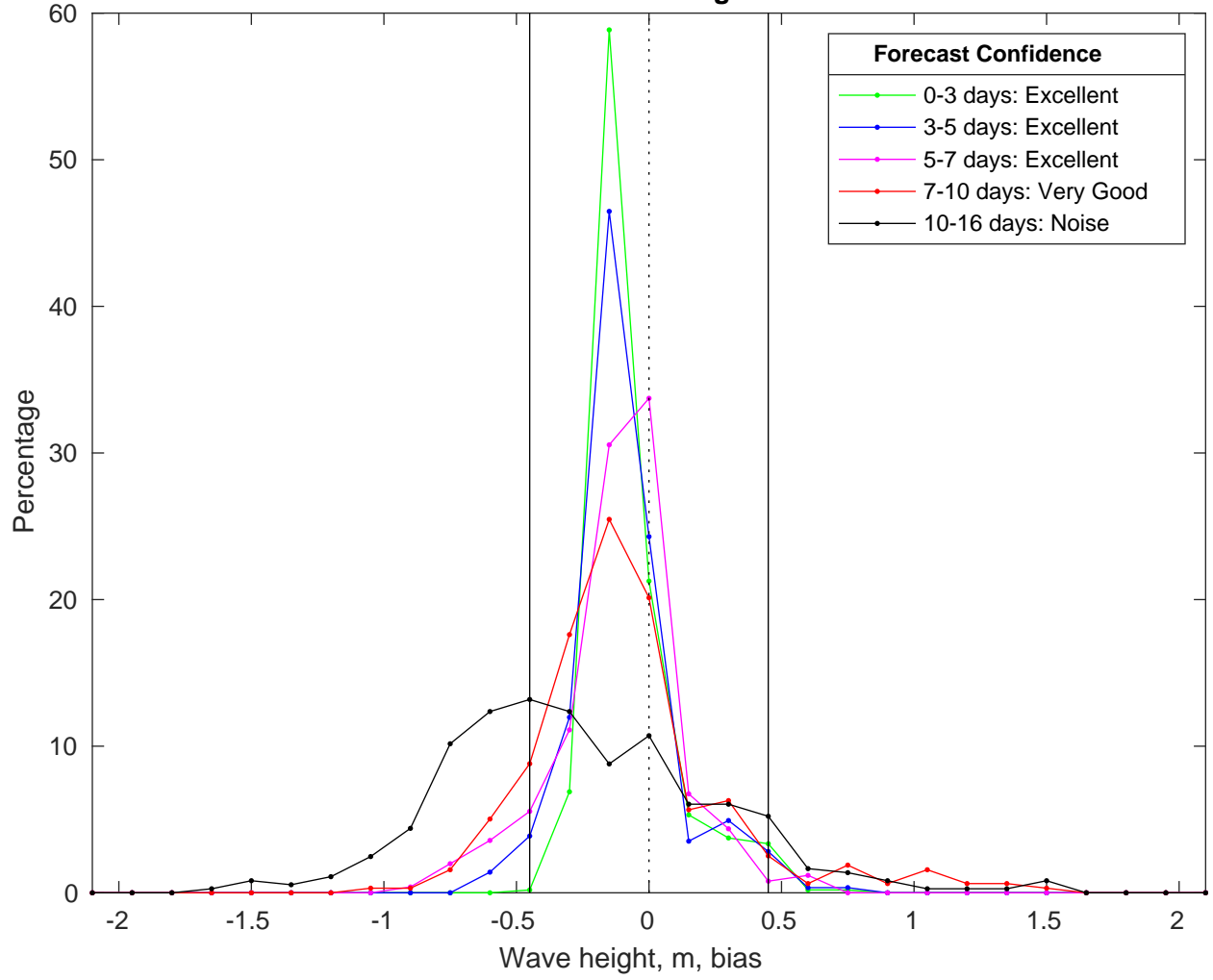
NDBC 42036 vs GFS Waves Bias Histogram: 17-Feb-2025
