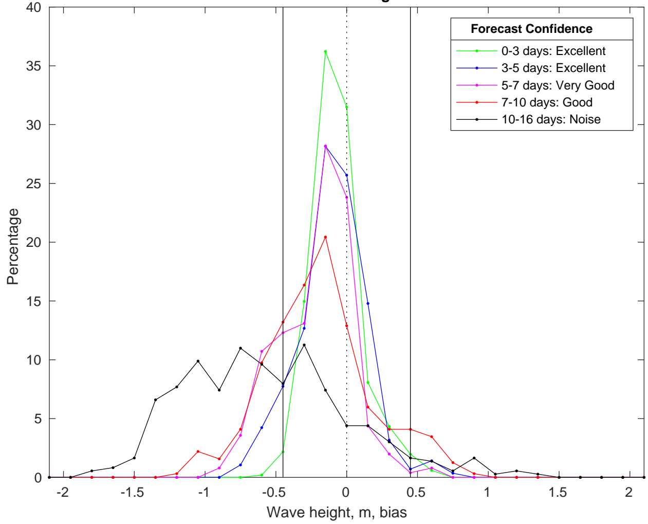
NDBC 42040 vs GFS Waves Bias Histogram: 17-Feb-2025
