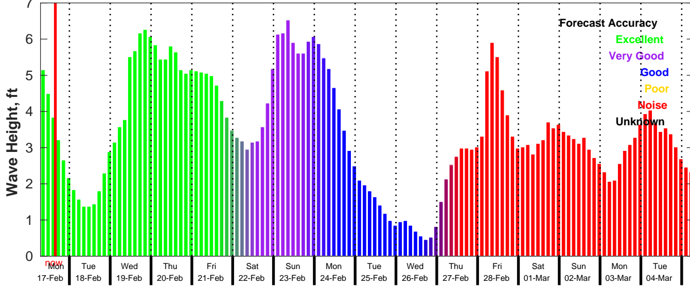
GFS Wave Forecast for NDBC 42040 from 17-Feb-2025 07:00:00 to 05-Mar-2025 07:00:00
