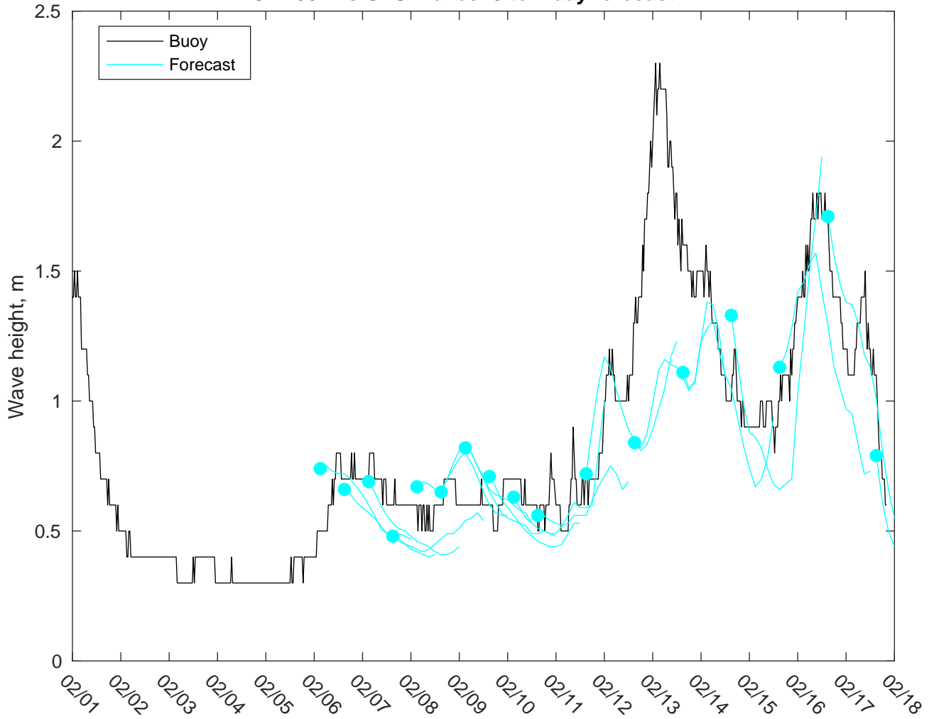
NDBC 42084 vs GFS Waves: 5 to 7 day forecast
