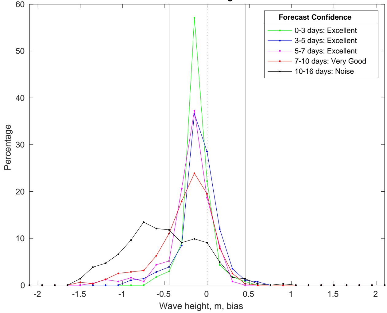
NDBC 42084 vs GFS Waves Bias Histogram: 17-Feb-2025
