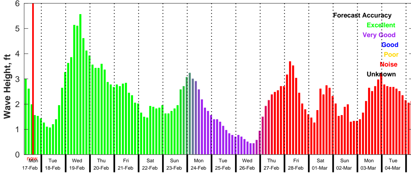
GFS Wave Forecast for NDBC 42084 from 17-Feb-2025 07:00:00 to 05-Mar-2025 07:00:00
