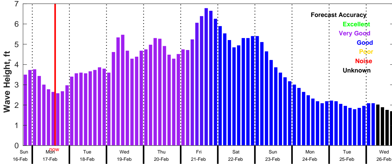
CMEMS Wave Forecast for NDBC 42092 from 16-Feb-2025 18:00:00 to 26-Feb-2025 18:00:00
