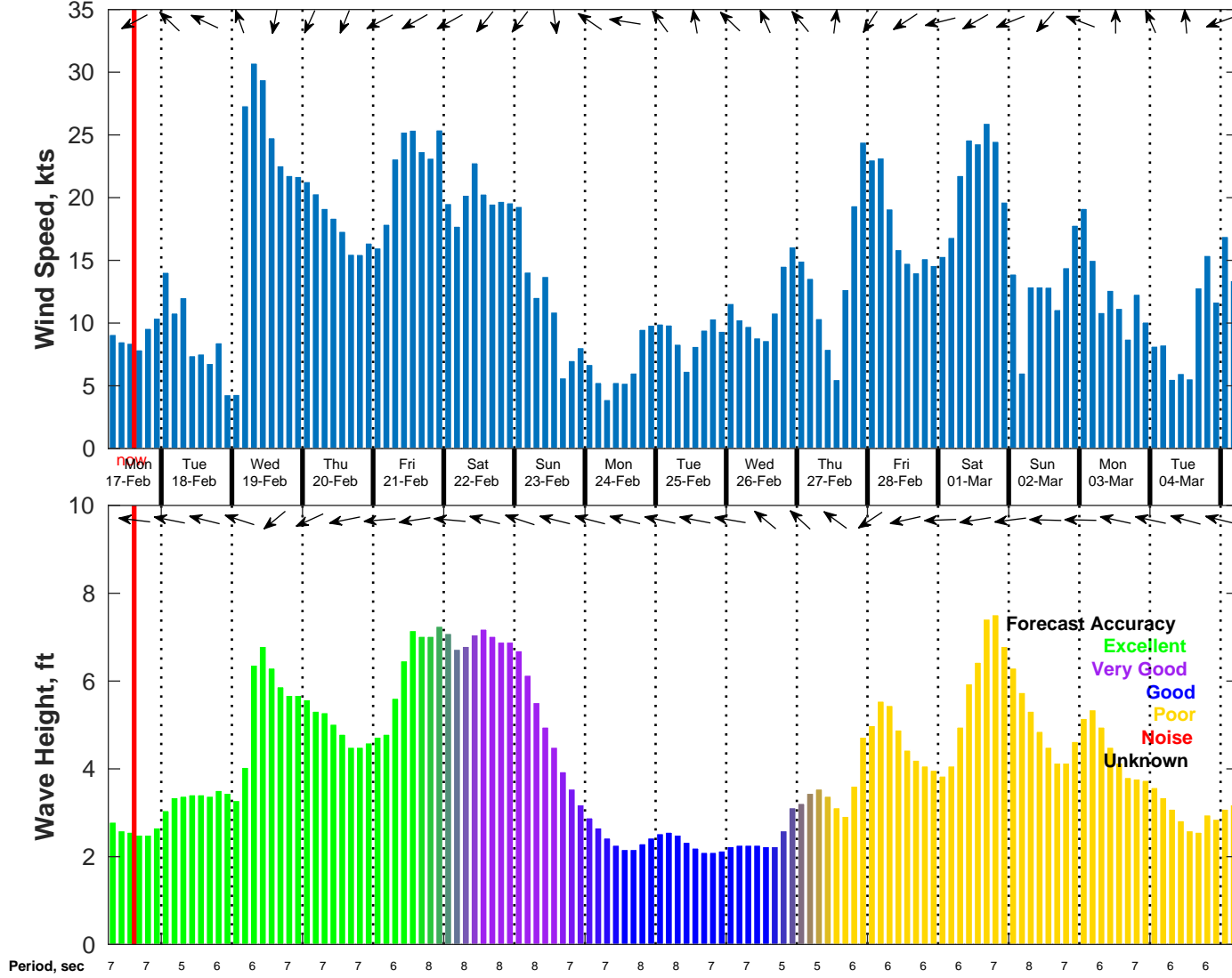
Wind & Wave Forecast for NDBC 42092 from 17-Feb-2025 06:00:00 to 05-Mar-2025 06:00:00
