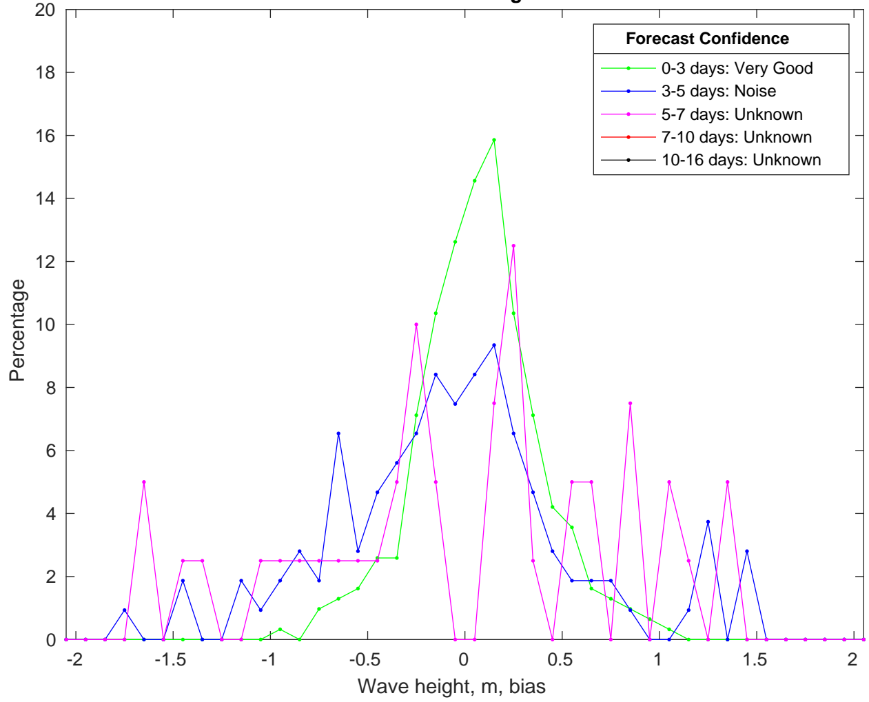
NDBC 44008 vs GFSWaves Bias Histogram: 18-Oct-2024
