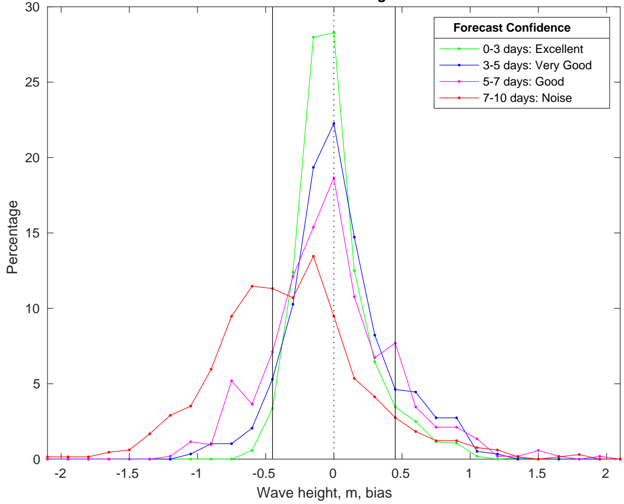
NDBC 46011 vs CMEMS Waves Bias Histogram: 17-Feb-2025
