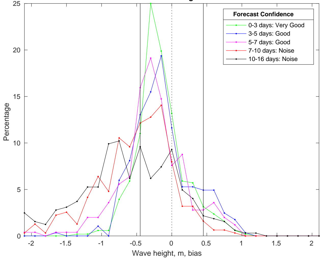
NDBC 46011 vs GFS Waves Bias Histogram: 17-Feb-2025
