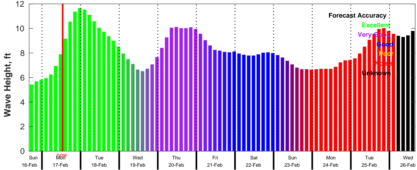
CMEMS Wave Forecast for NDBC 46011 from 16-Feb-2025 16:00:00 to 26-Feb-2025 16:00:00
