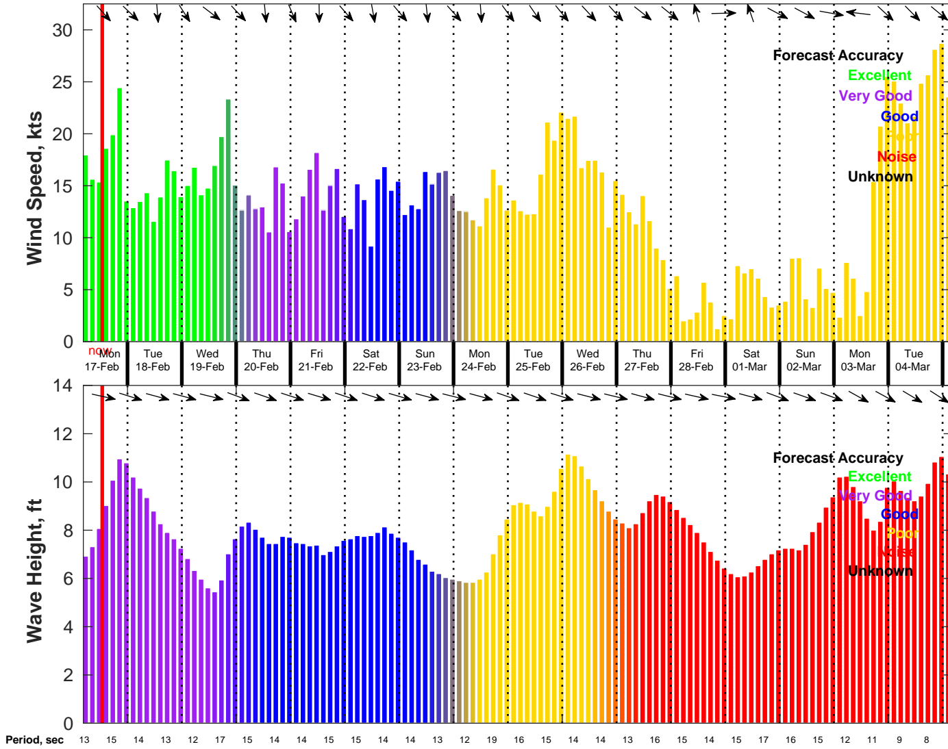
Wind & Wave Forecast for NDBC 46011 from 17-Feb-2025 04:00:00 to 05-Mar-2025 04:00:00
