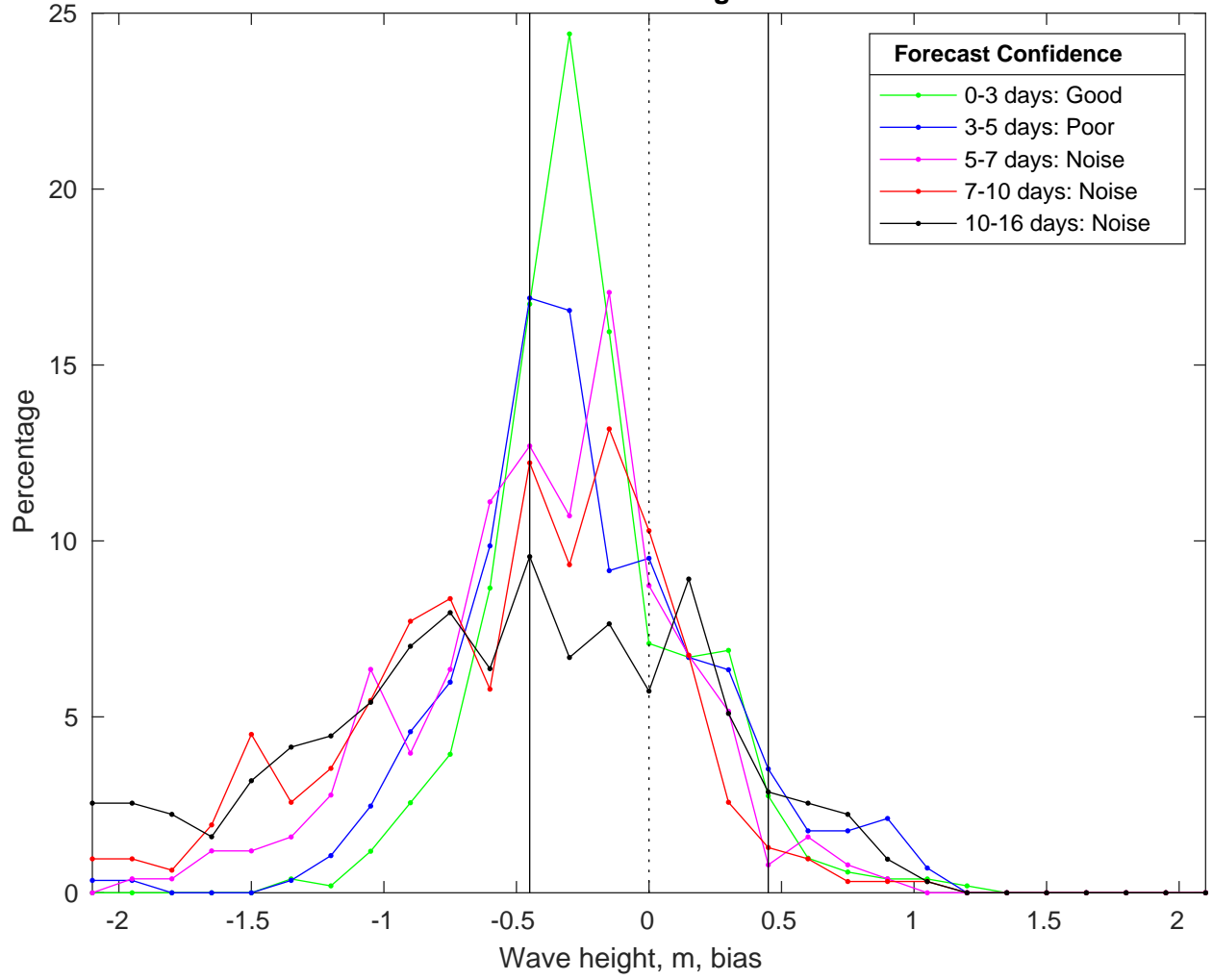
NDBC 46028 vs GFS Waves Bias Histogram: 17-Feb-2025
