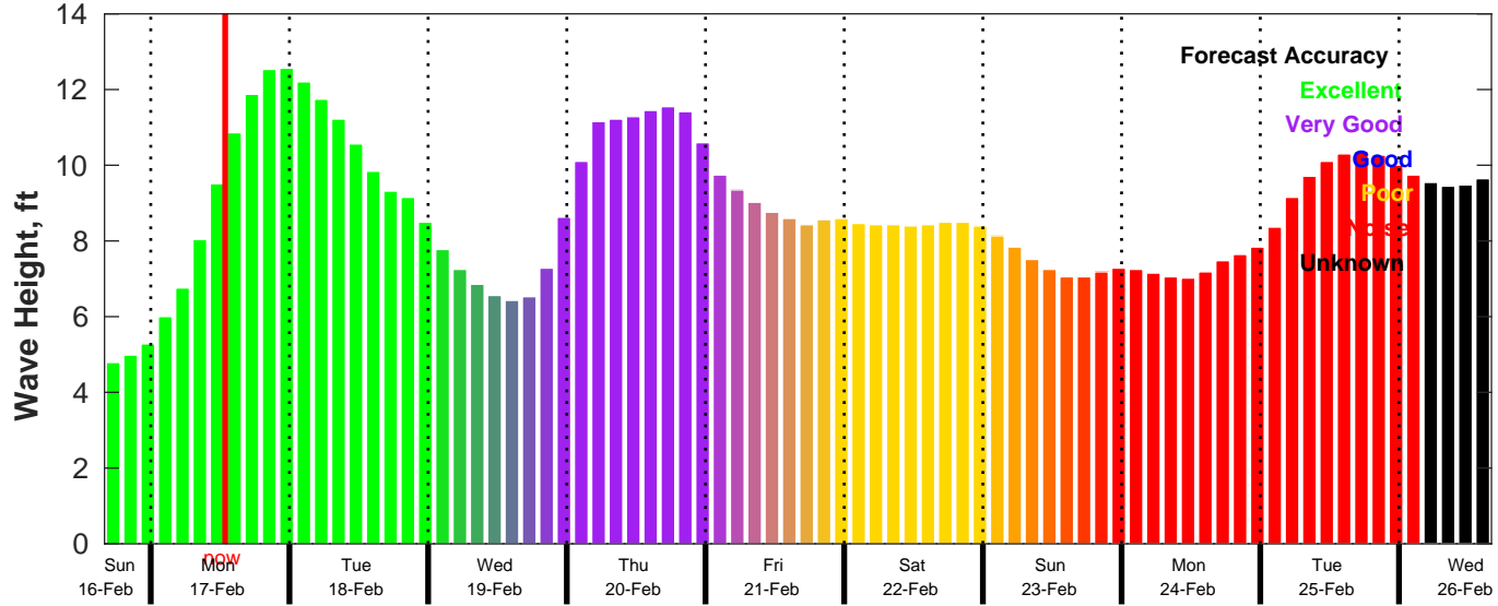
CMEMS Wave Forecast for NDBC 46028 from 16-Feb-2025 16:00:00 to 26-Feb-2025 16:00:00
