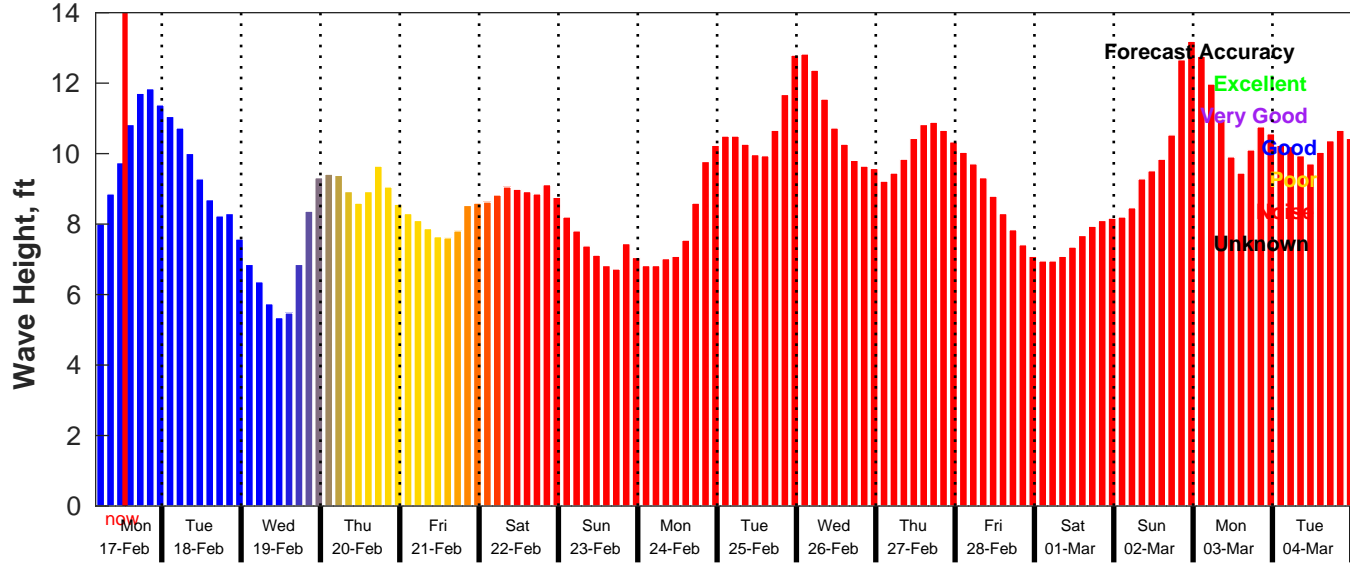
GFS Wave Forecast for NDBC 46028 from 17-Feb-2025 04:00:00 to 05-Mar-2025 04:00:00
