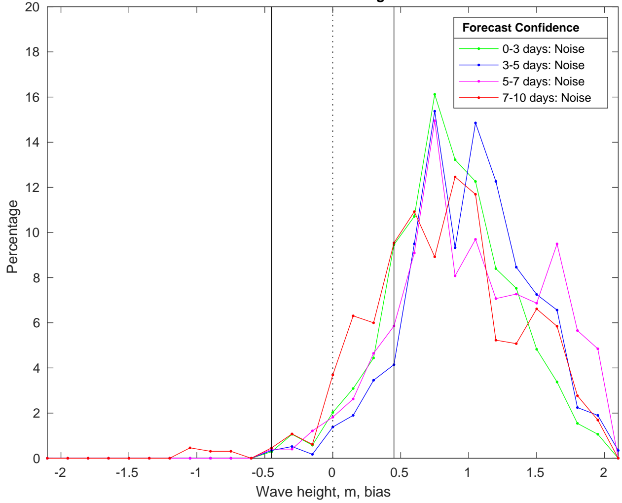
NDBC 46053 vs CMEMS Waves Bias Histogram: 17-Feb-2025
