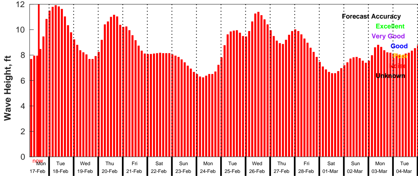
GFS Wave Forecast for NDBC 46053 from 17-Feb-2025 05:00:00 to 05-Mar-2025 05:00:00
