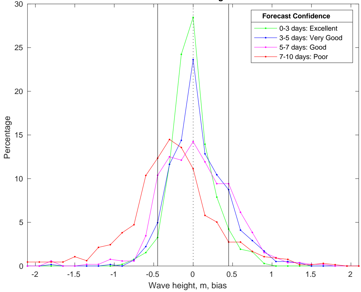
NDBC 46054 vs CMEMS Waves Bias Histogram: 17-Feb-2025
