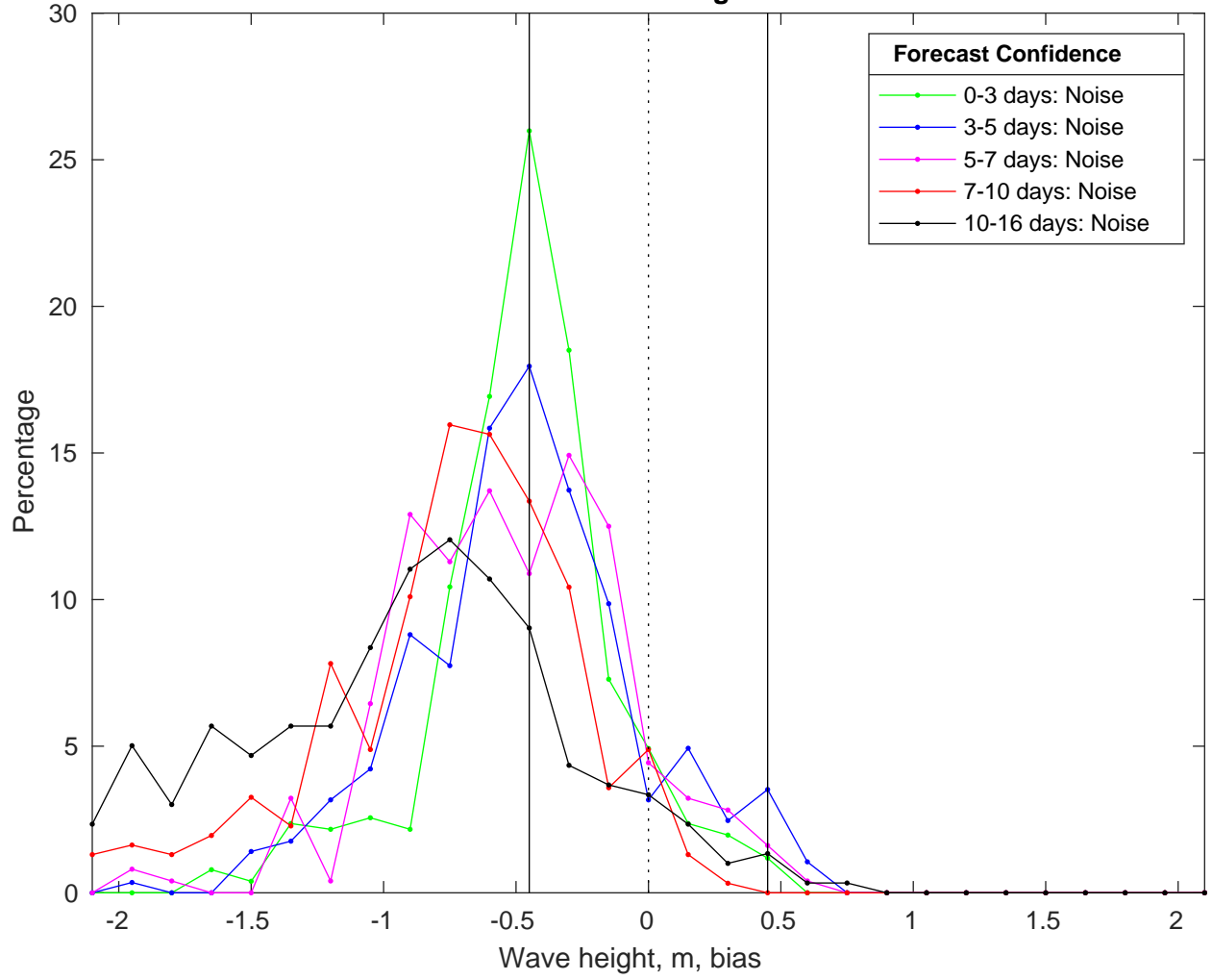
NDBC 46054 vs GFS Waves Bias Histogram: 17-Feb-2025
